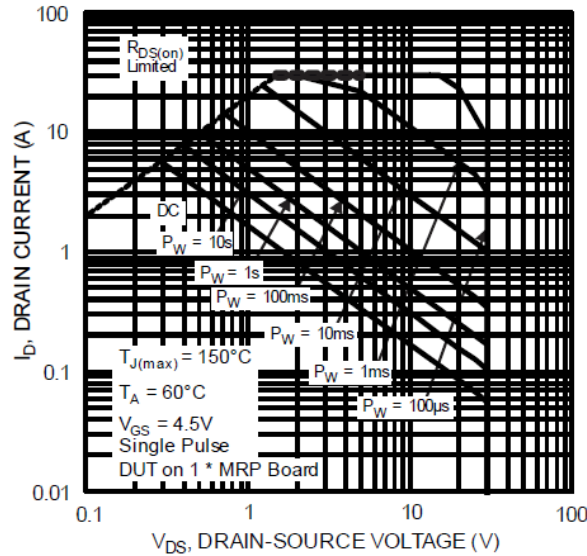
Figure 4 Safe Operating Area (SOA) for DMN3027LFG
