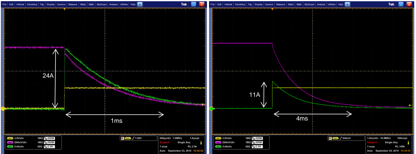
Figure 7 Elevated temperature measurements (approx. T_a=70^\circ\text{C} ). Left curves = 24A peak current discharge through DMN3027LFG channel resistance only (200μs/div) Right curves = 11A peak current discharge through DMN3027LFG and 50mΩ series resistor (1ms/div)
