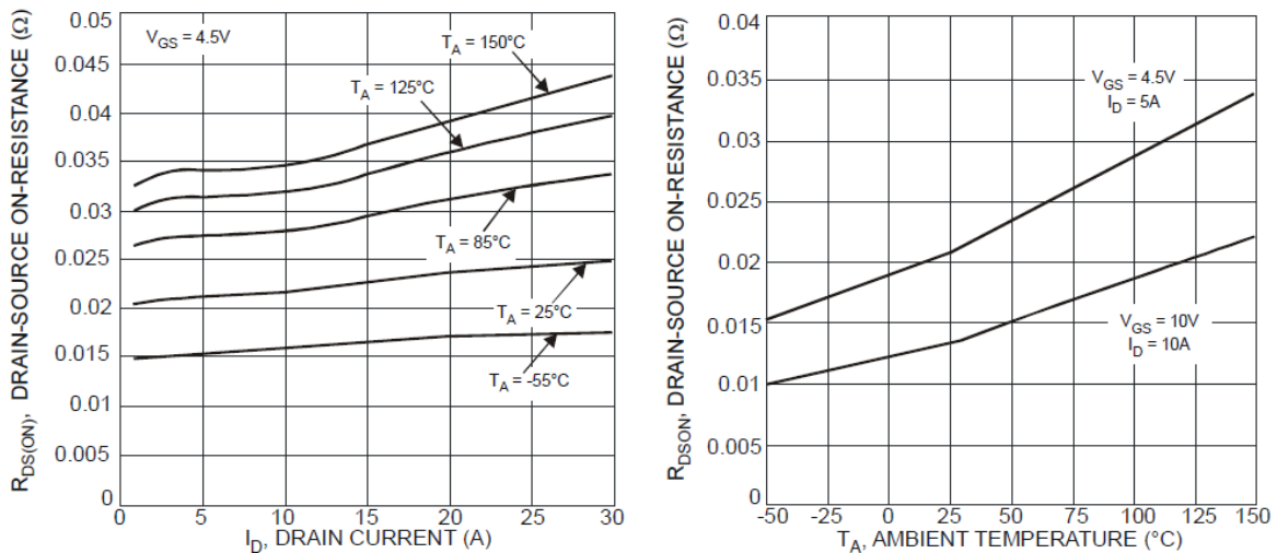
Figure 5 On-resistance temperature response of DMN3027LFG
