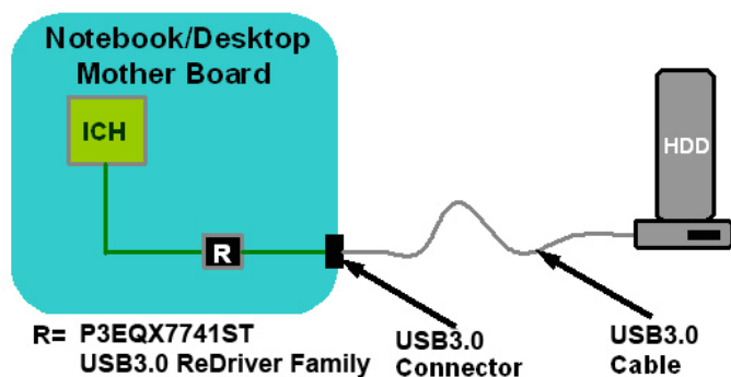
Figure 1 Typical Application in Notebook and Desktop
