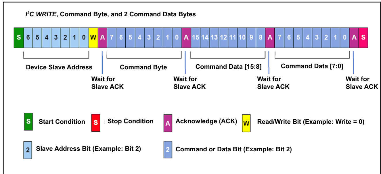
Figure 17: I 2 C Command Format
