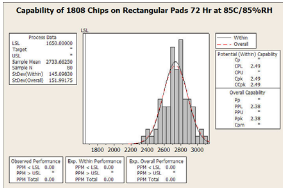
1808 Chip Capacitors Mounted on Boards Breakdown Capability after 72 Hours of 85°C/85%RH Exposure
