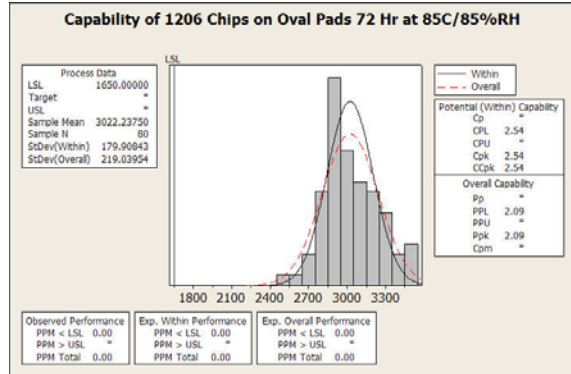
1206 Chip Capacitors Mounted on Boards Breakdown Capability after 72 Hours of 85°C/85%RH Exposure
