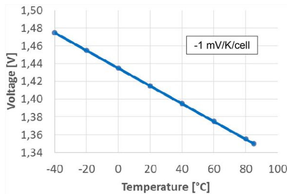
Fig. 1 - Charging voltage as a function of temperature
