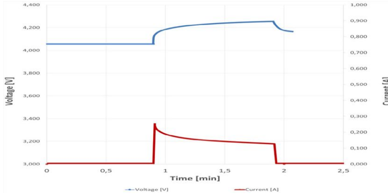
Fig. 6a - First maintenance charge pulse (1 minute) after 6 h (example 90 F 4.2 V)
