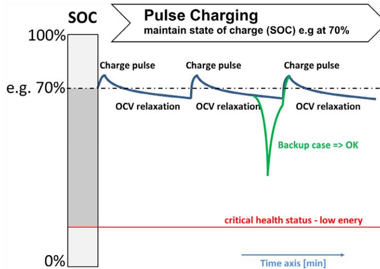
Fig. 5 - Typical maintenance charge over time - charge pulses keep SOC on a defined high level. OVC relaxation is dependent on the load situation and self-discharge. For a typical backup, SOC has to be high enough to supply the required energy.
