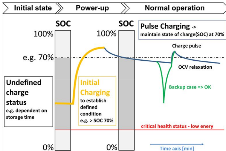
Fig. 7 - Typical power-up and normal operation cycles. Initial charging is necessary in order to establish the desired SOC level for normal operation.
