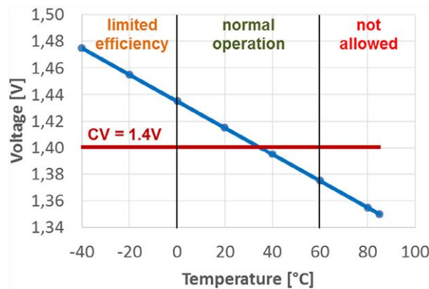
Fig. 2 - Charging with 1.40 V per cell over temperature range
