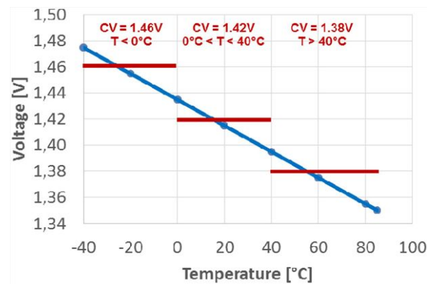
Fig. 3 - Stepwise approximation with three voltage levels
