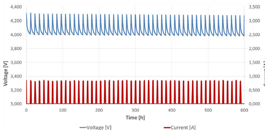
Fig. 6 - 196 HVC 90 F maintenance charge 1 minute every 12 hours at 45 °C
