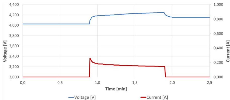
Fig. 8 - The first 15 minutes of initial charge (example 90 F, 4.2 V)
