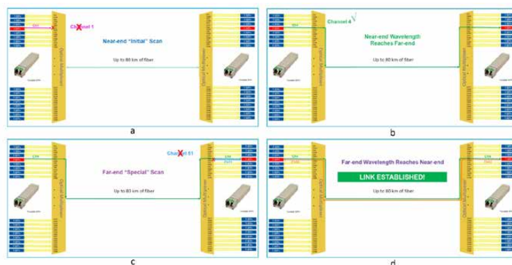
Figure 4(a-d): Flexitone™ self-tuning process for duplex T-SFP+ transceivers.
