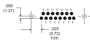
15 Contacts
