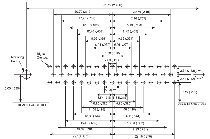
50 Contacts
