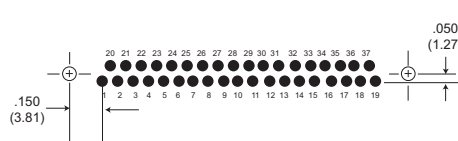
37 Contacts
