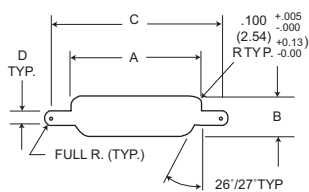
Figure 2 Rear Mounting
