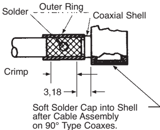
90° Coaxial
