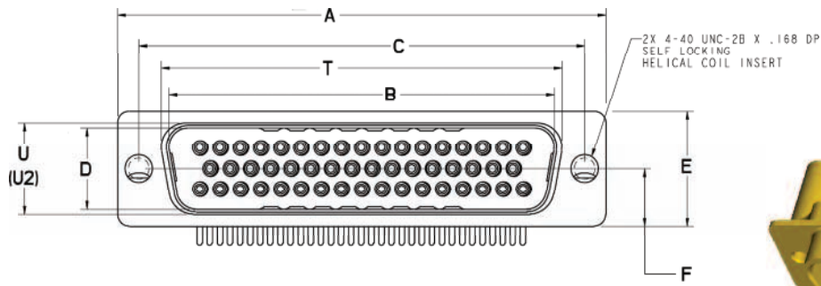
Plug - Pin
