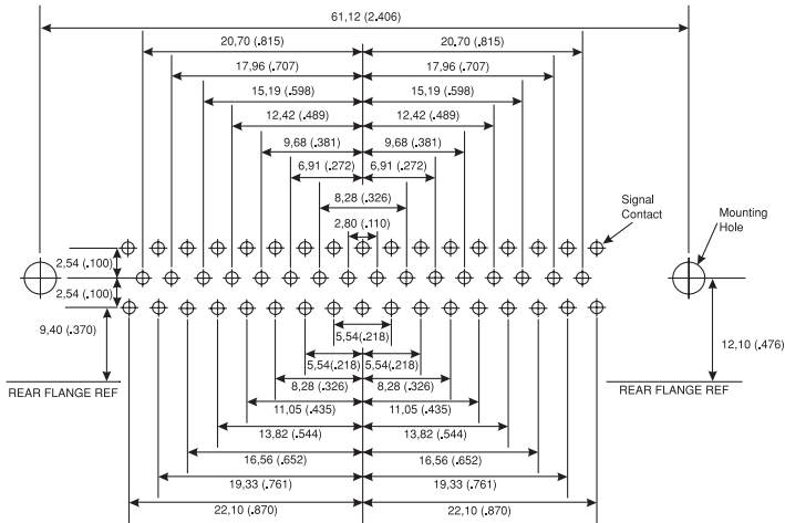
50 Contacts
