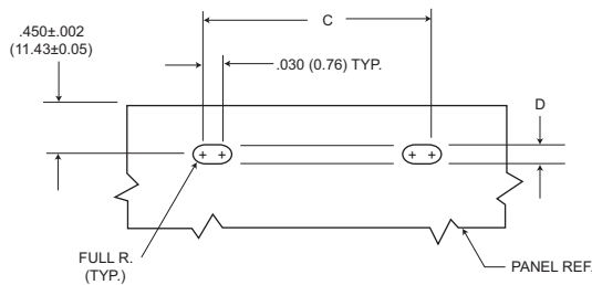
Figure 3 Edgeboard Mounting
