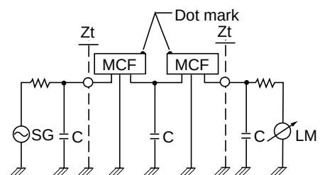
4-POLE MCF Zt: Terminating Impedance
