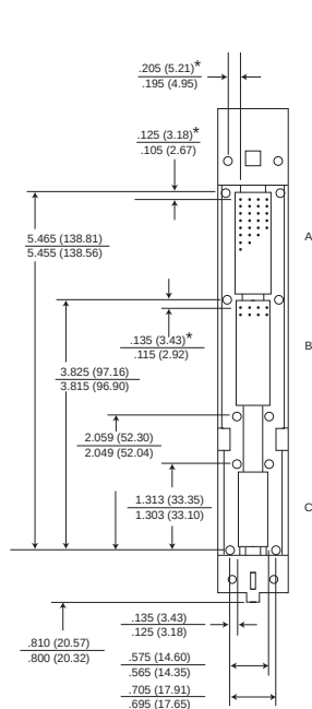
Retainer Plate Detail
