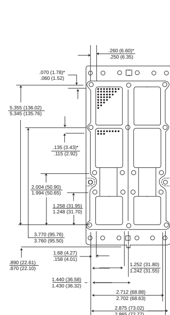
Retainer Plate Detail
