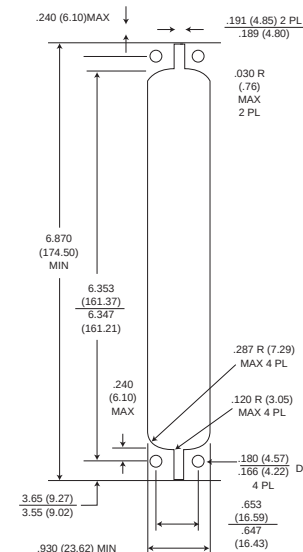
Panel Cutout
