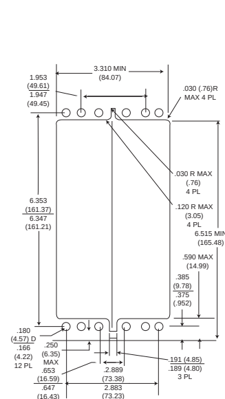
Panel Cutout
