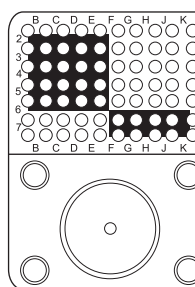
71W1 70 #22 1 #1 COAX
