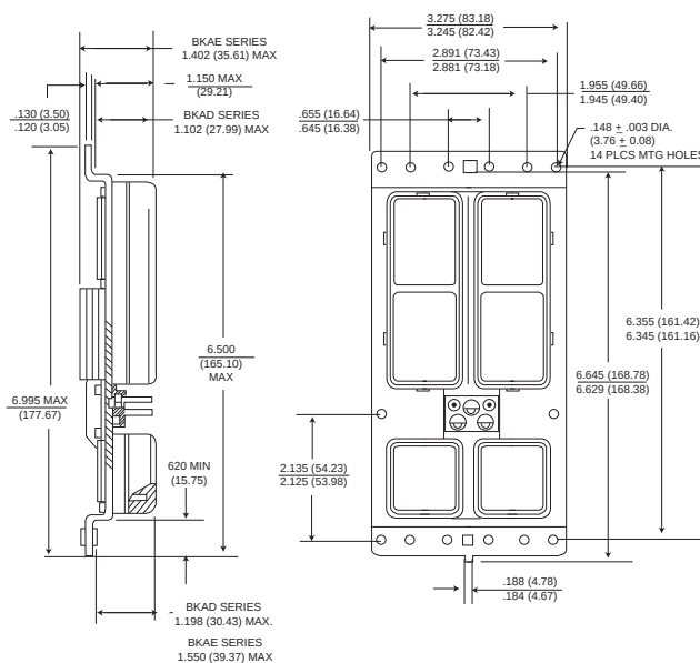
Size 3 Plug
