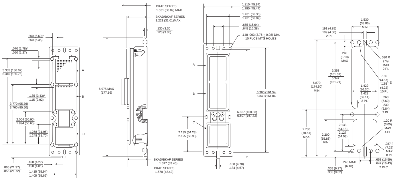
Retainer Plate Detail
