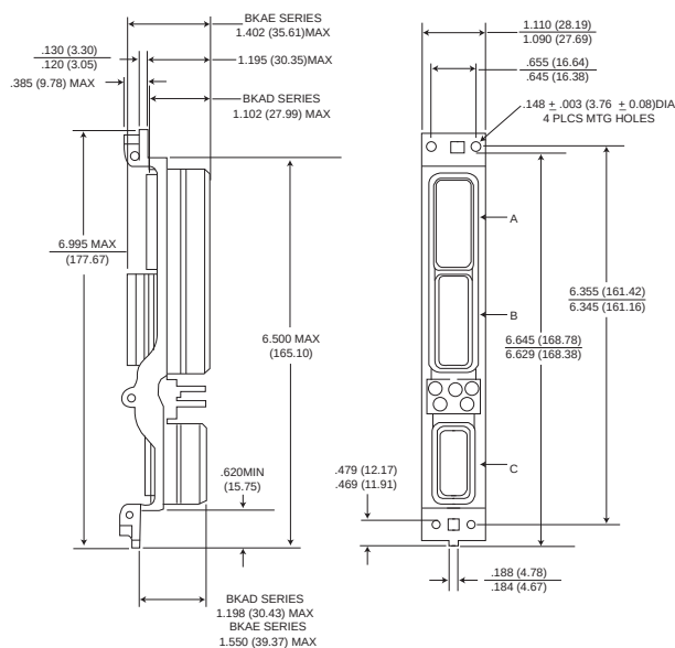
Size 1 Plug
