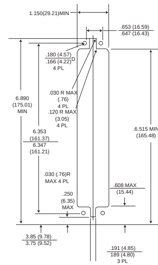
Panel Cutout
