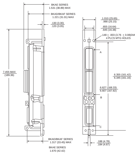
Size 1 Receptacle
