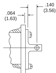
-0201 Modification Tabs for attaching J/S
