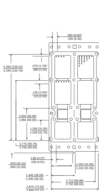
Retainer Plate Detail
