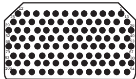
A106 106 #22 1000
