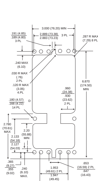
Panel Cutout
