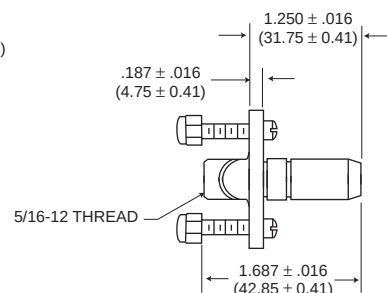
P/N 013837-0013 DF 5/16-12 Quad Lead Thread
