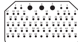
67M 64 HD #20, 3 #16 1000
