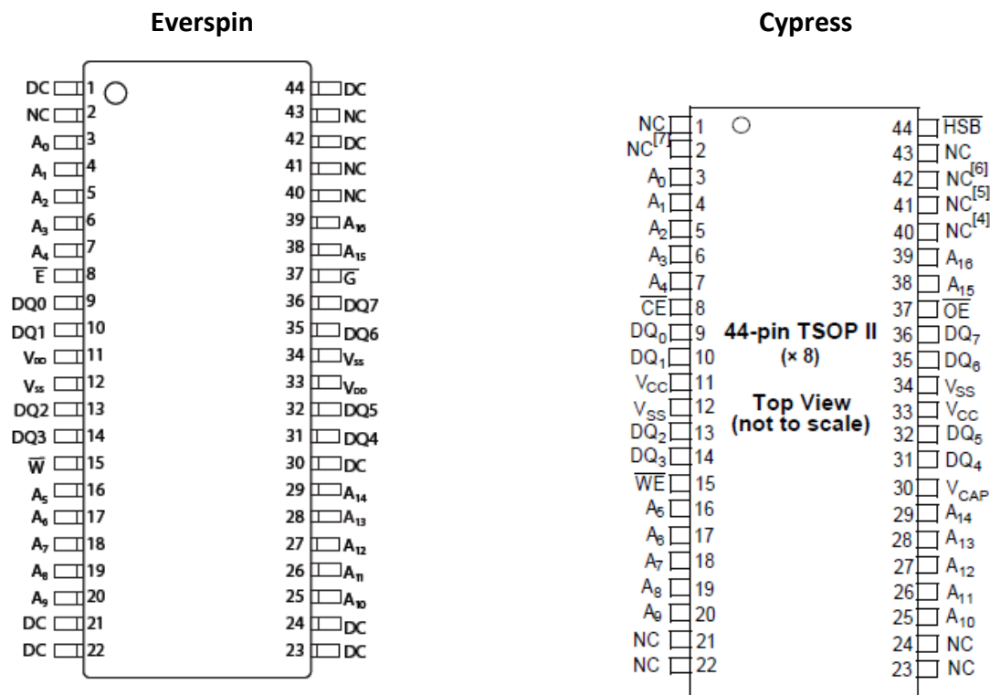
Figure 1 - Pin function comparison between MRAM and nvSRAM, 44 pin TSOP2 package
