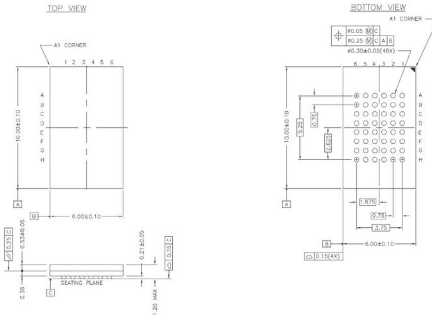
Figure 4 - Everspin FBGA package dimensions
