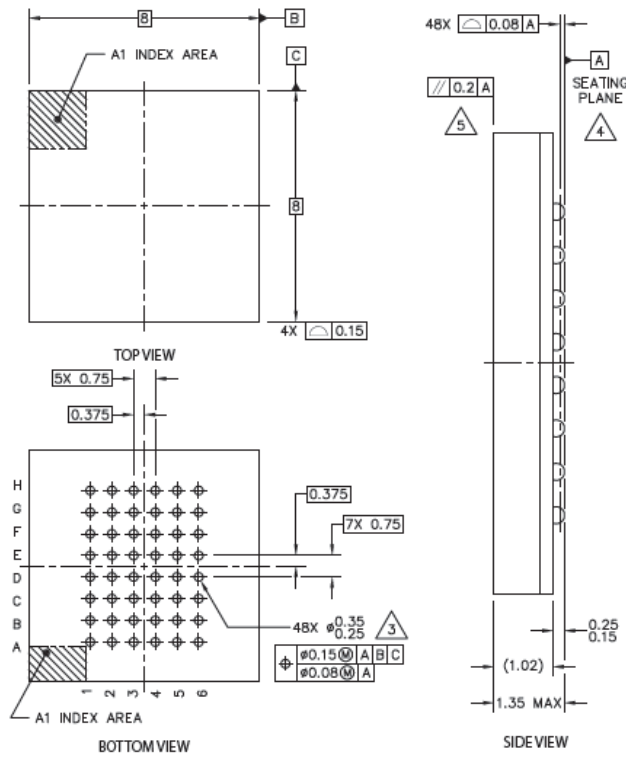
Figure 4 - Everspin FBGA package dimensions
