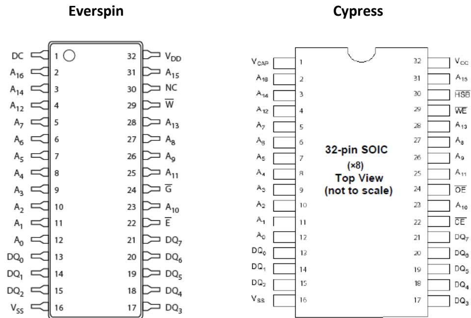
Figure 2 - Pin function comparison between MRAM and nvSRAM, 32 pin SOIC package
