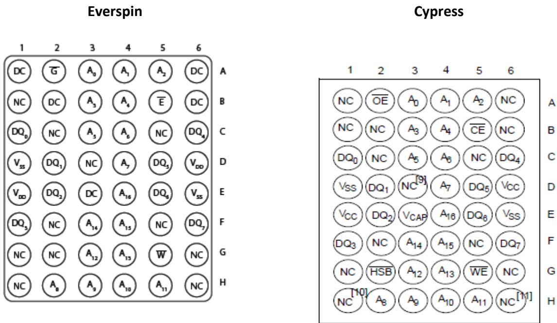
Figure 3 - Pin function comparison between MRAM and nvSRAM, 48 FBGA package
