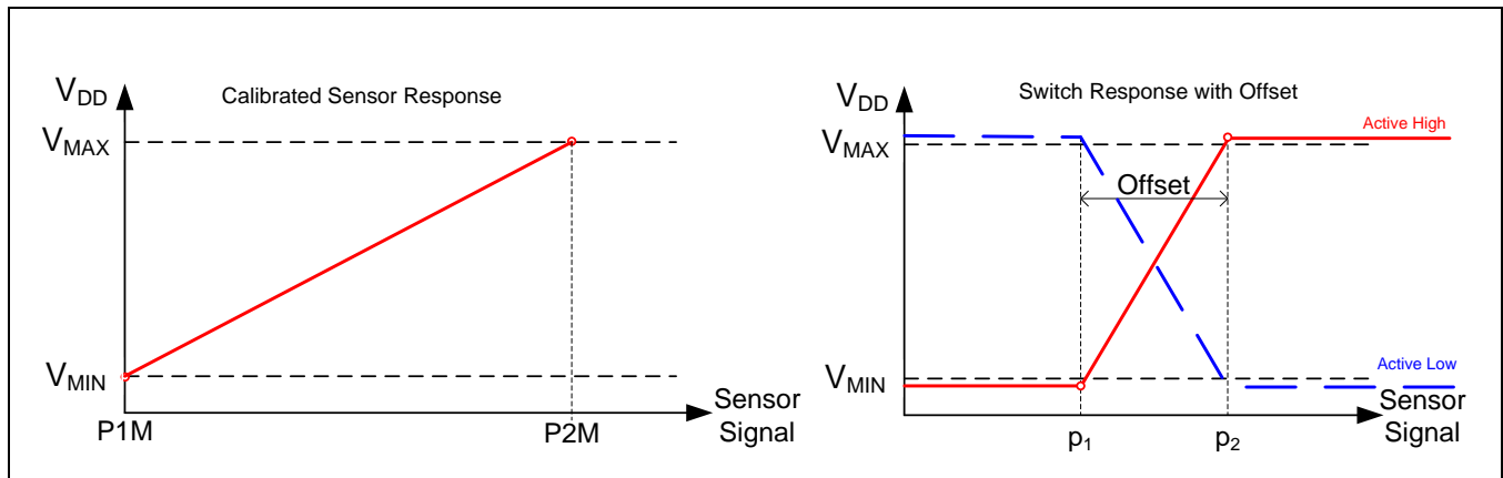
Figure 2.2 Switch Implementation
